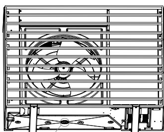
Hole in bottom panel of outdoor unit
