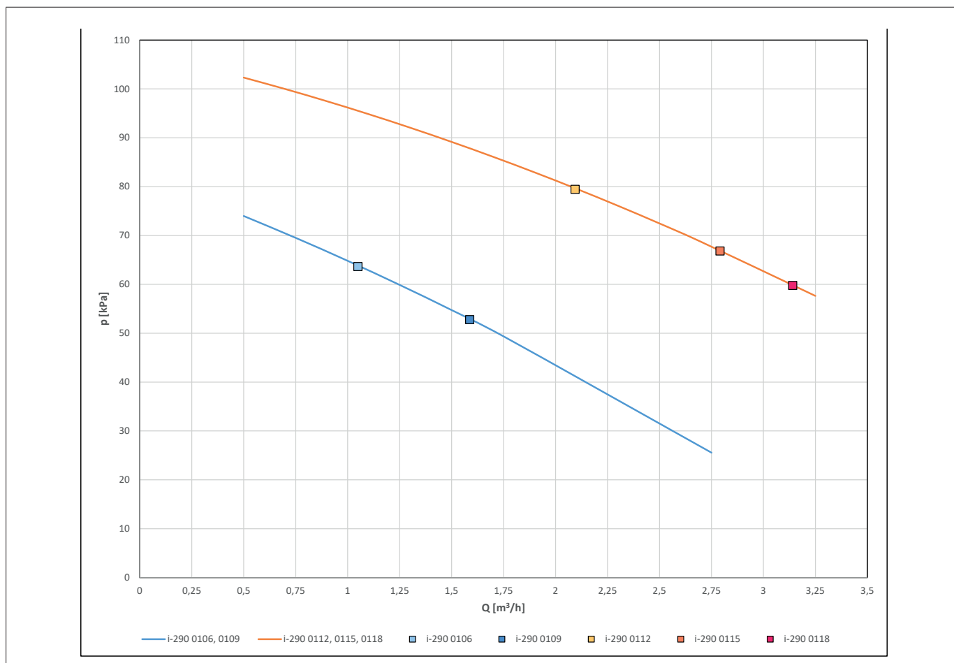
p [kPa] Useful head Q [m³/h] Water flow rate
